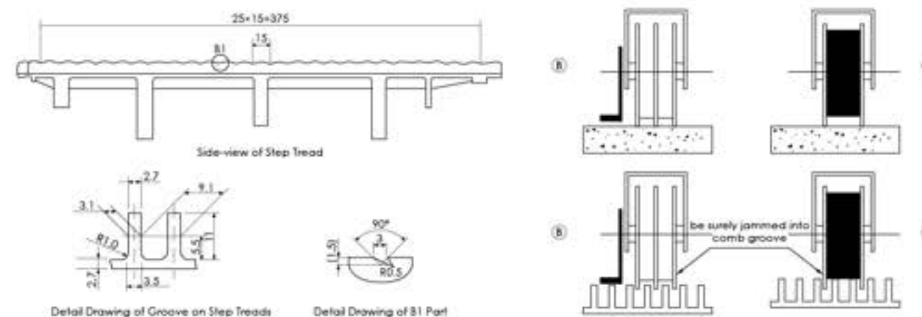
Sectional View of Step Treads on Moving Walk
